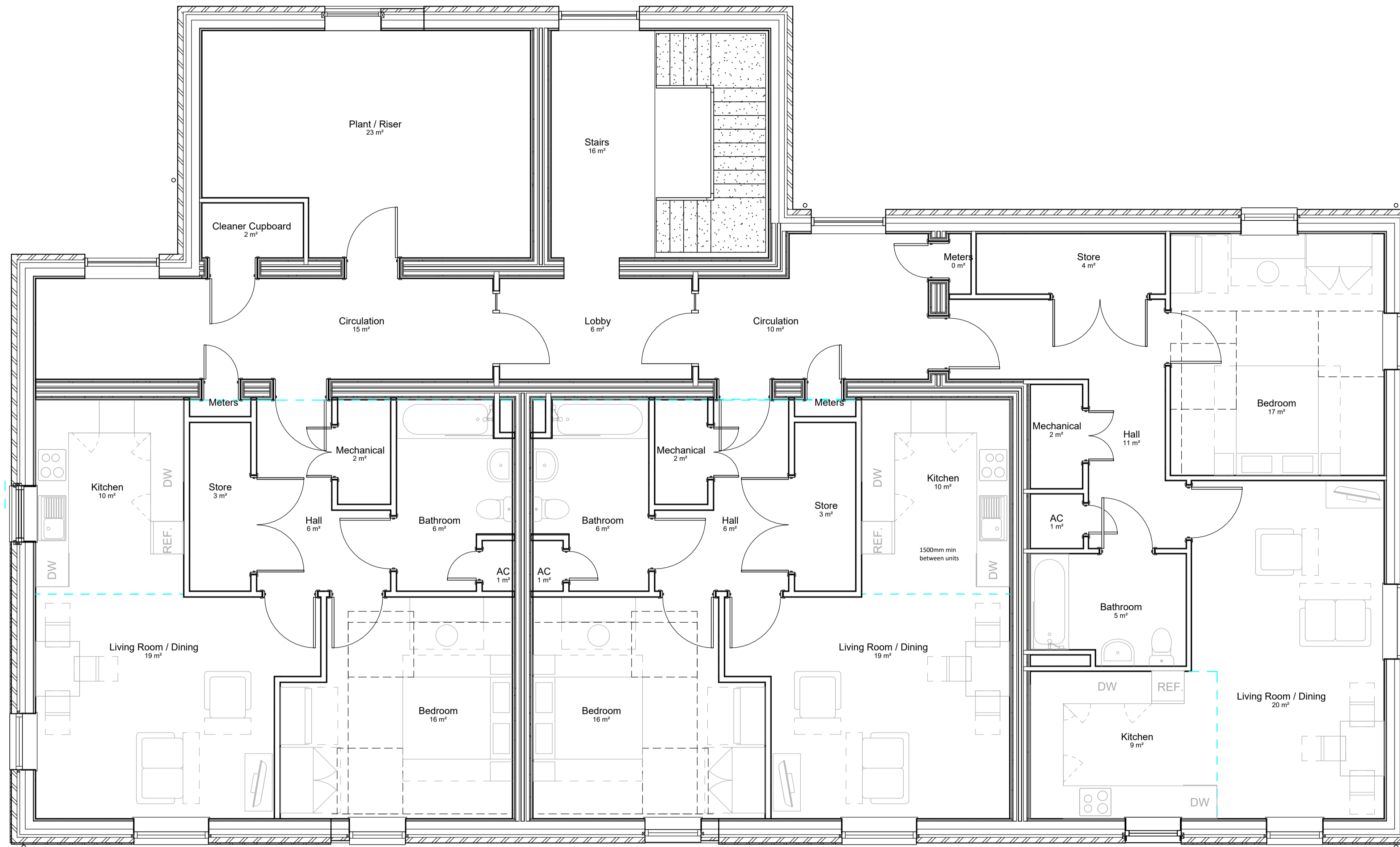
Second Floor 1 : 50
